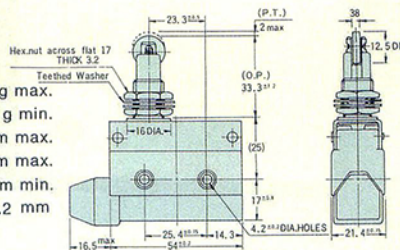
Panel mount roller plunger
